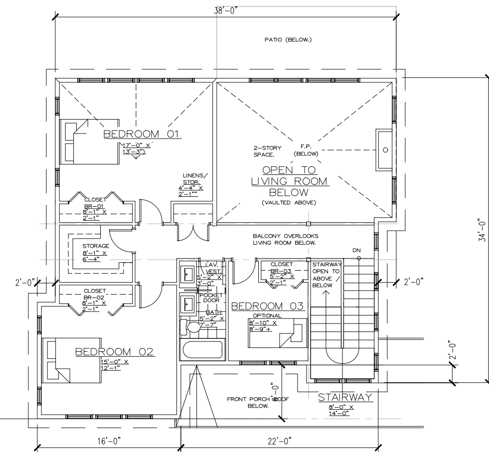
2 2nd Floor Plan SK-01.2 SCALE: 3/32" = 1'-0"
