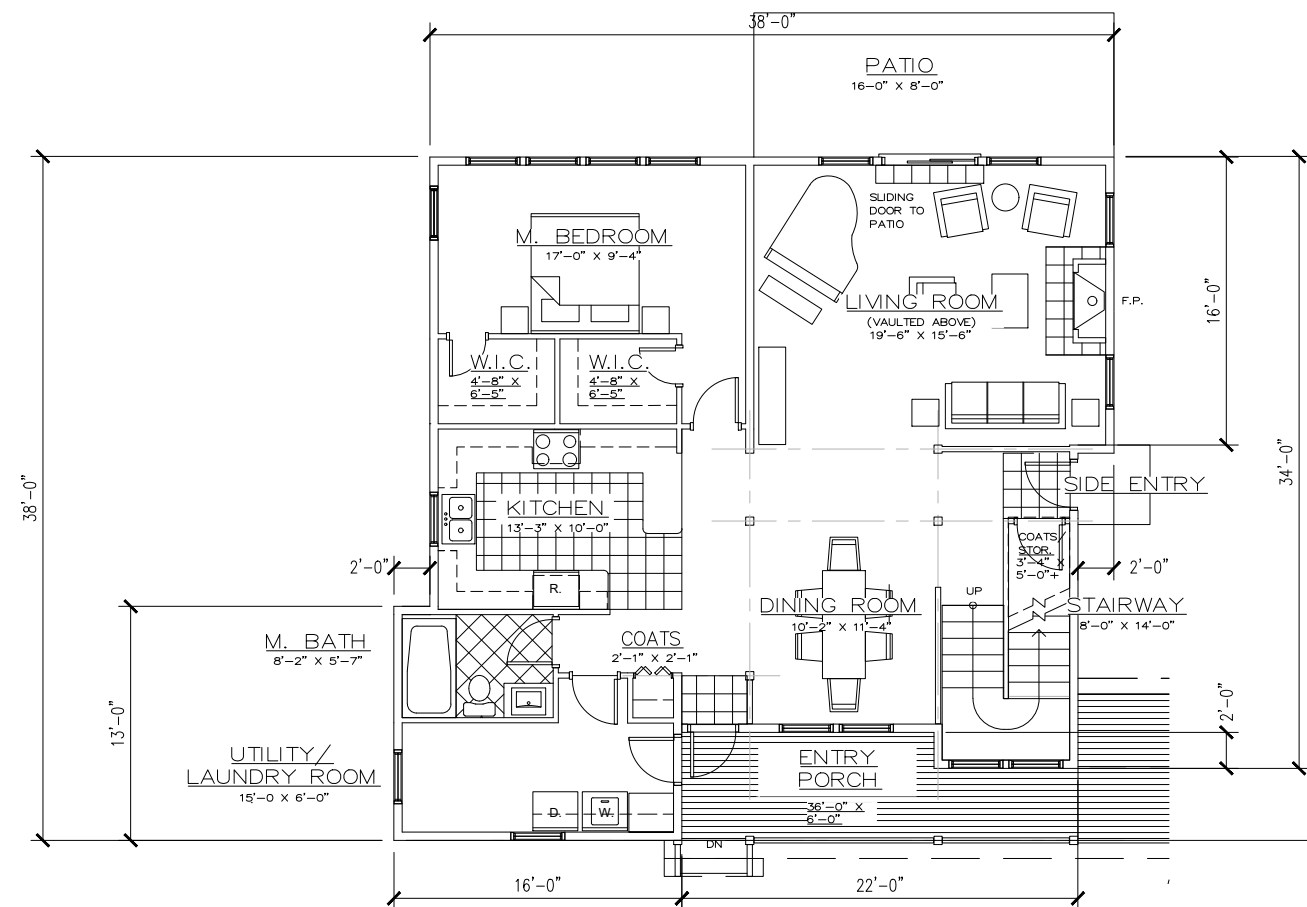
1 1st Floor Plan SK-01.2 SCALE: 3/32" = 1'-0"
