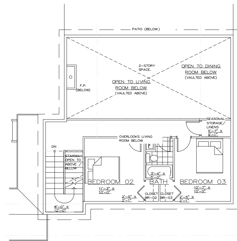
2 2nd Floor Plan SK-02.2 SCALE: 3/32" = 1'-0"
