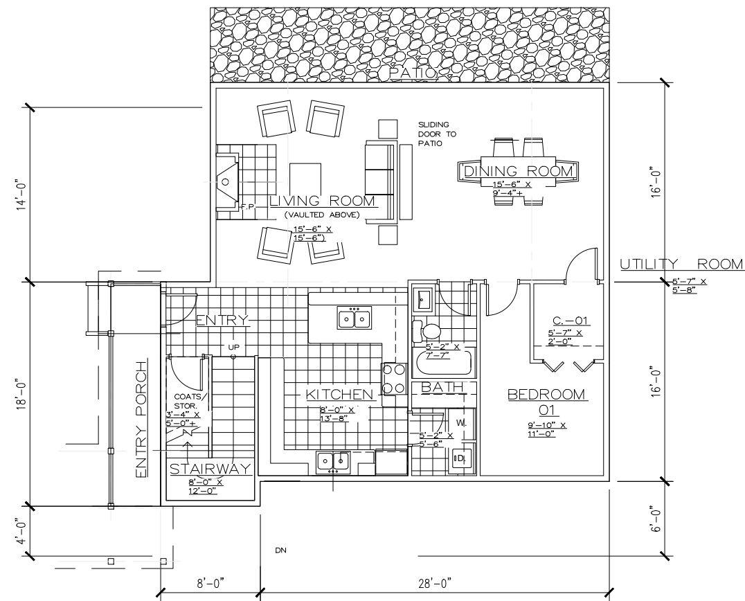
1 1st Floor Plan SK-02.2 SCALE: 3/32" = 1'-0"
